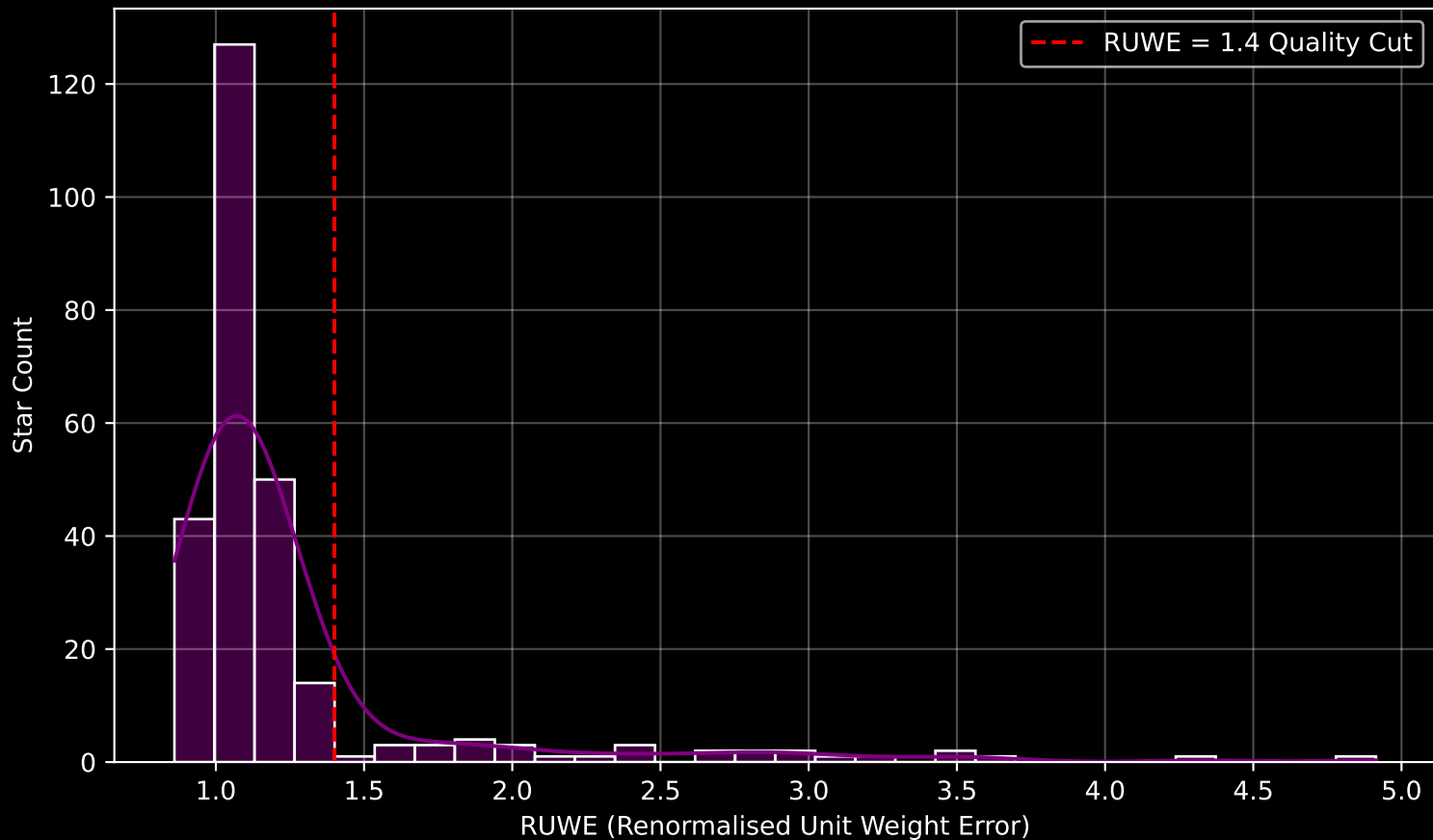
GALAH DR4 Field [1741] RUWE Distribution (n= 266)
