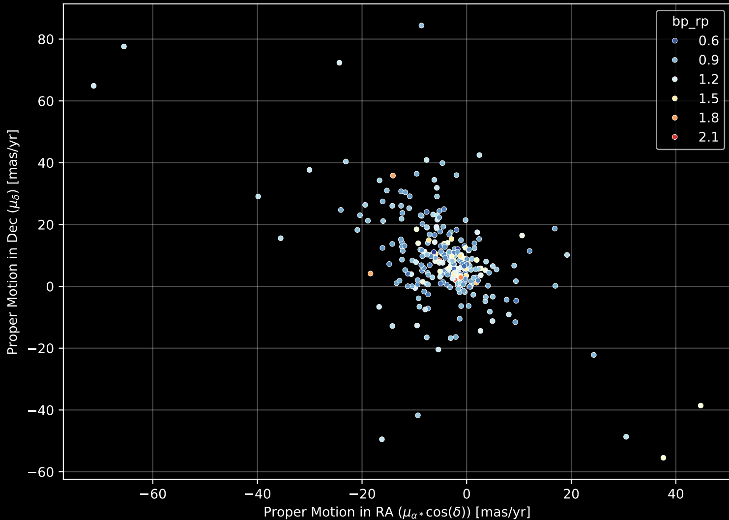
GALAH DR4 Field: [1741] Proper Motion Diagram (n= 277)
