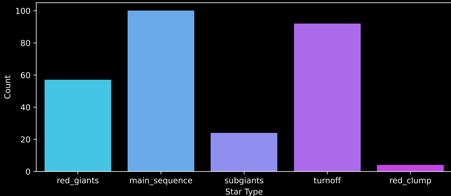
GALAH DR4 Field: [1741] Count plot of Star Type
