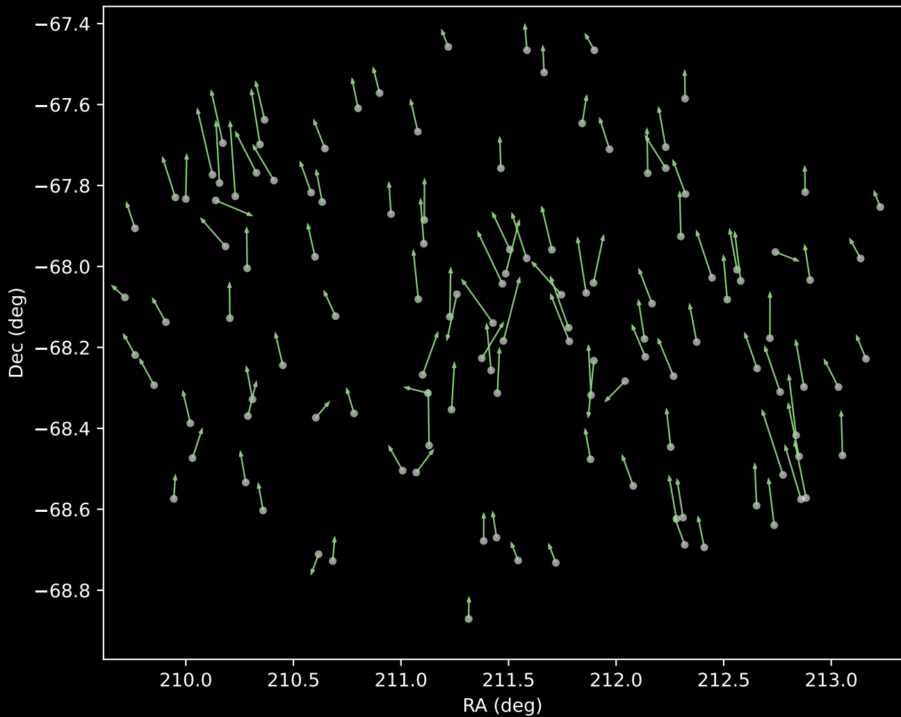
GALAH DR4 Cluster 5 Proper Motion Vectors (n=122)
